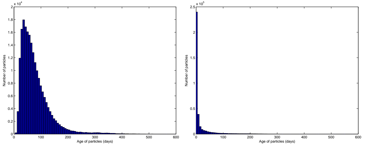
Figure 3.3: On the right the histogram presents age for particles reaching the Balearic channel and on the left it presents the age of particles reaching the Corsican sections. The histograms present the repartition of the particles age when they are intercepted. Each bar represents the number of particles intercepted during a 7-days period.
