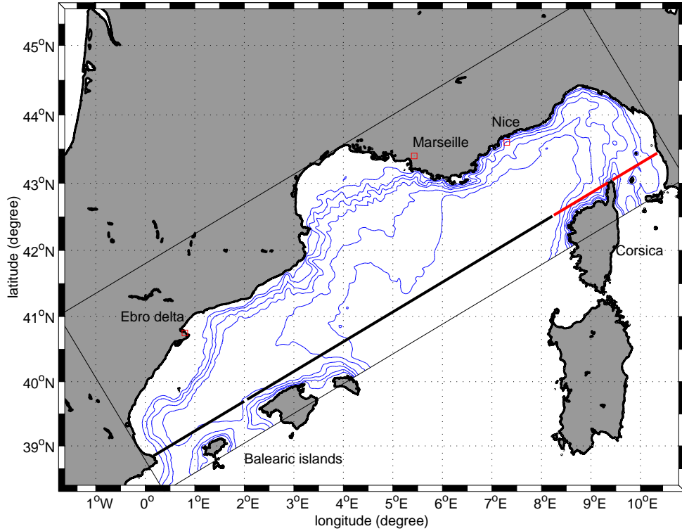
Figure 2.1: Domain used for the Lagrangian diagnostic. The red line represents the section on initialization for the upstream diagnostic. The black line represents the sections of interception for this diagnostic. The isobaths presented on this figure are : -100 -200 -500 -1000 -2000 and -2500 meter
