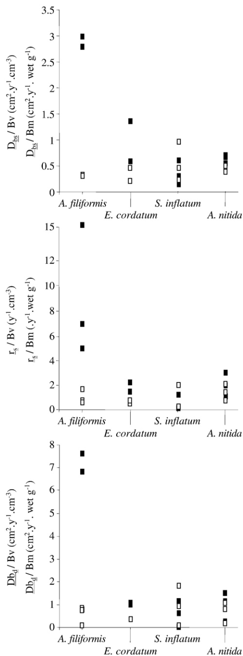
Fig. 4. Biodiffusion ( D_{bs} and D_{bd} ) and biotransport ( r_s ) coefficients per wet biomass (solid symbol) and per biovolume (open symbol) calculated for the four studied macrobenthic species. D_{bs} and r_s : coefficients for the surface tracers; D_{bd} : coefficient for the deep tracers. Values are individual points for triplicate observations.
