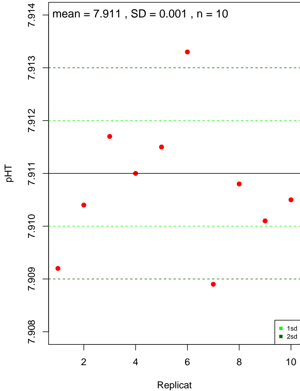
CAST 20 NISKIN 3
