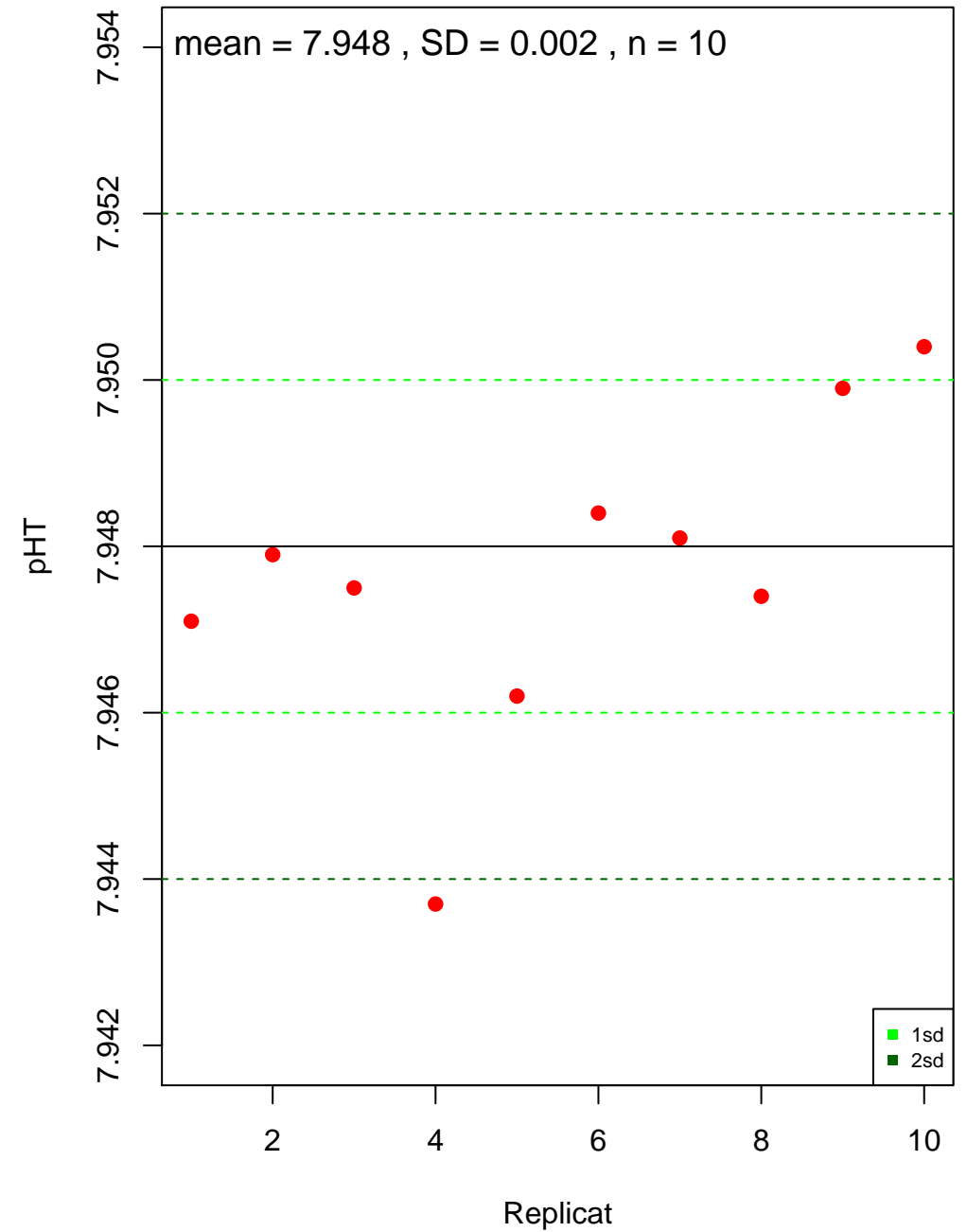
CAST 20 NISKIN 20
