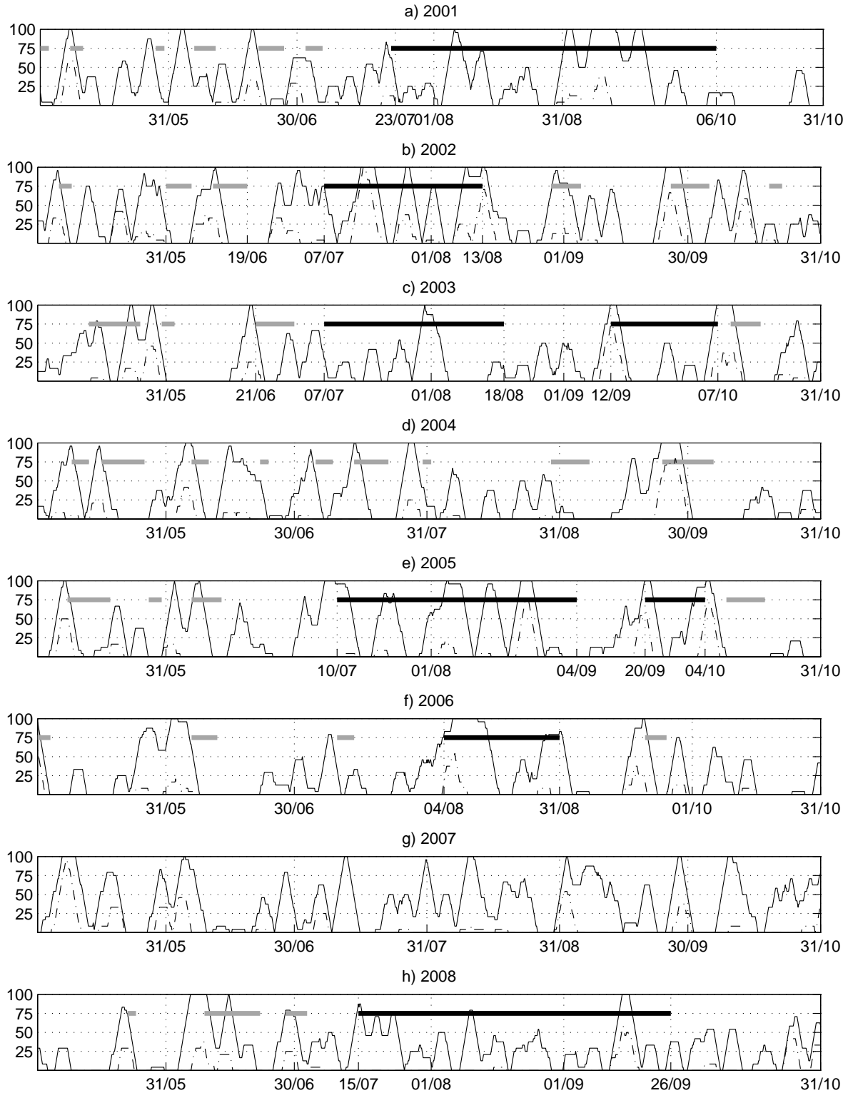
Figure 7. Temporal evolution of northwesterly expressed as a percentage of all wind, with a 3 day moving average, (continuous line: northwesterly intensity \geq 8 \text{ ms}^{-1} ; dotted line: \geq 14 \text{ ms}^{-1} ) from May 1 to October 31 for each year. The presence of ‘long-life’ eddies is indicated by
