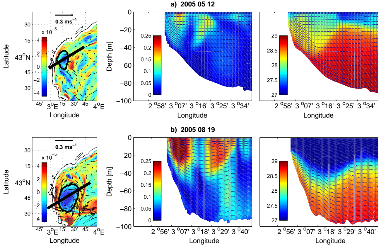
Figure 9. Left: relative vorticity at 20 m depth, current velocity fields and eddy contour; black line marks the eddy cross-section; Middle: Vertical transect of current intensity [ms -1 ]; Right: Vertical transect of density for a): May 12 and b): August 19, in 2005.
